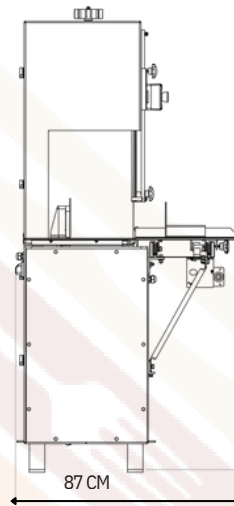
VISTA FRONTAL
