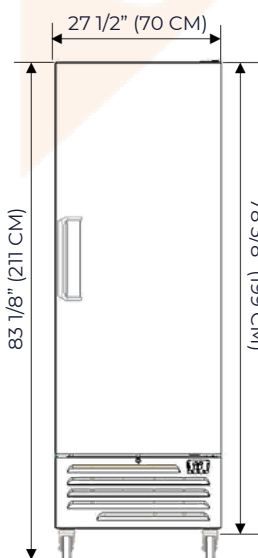
VISTA FRONTAL
