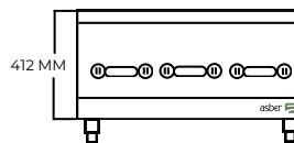
VISTA FRONTAL
