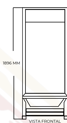
VISTA FRONTAL
