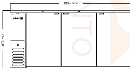
VISTA FRONTAL
