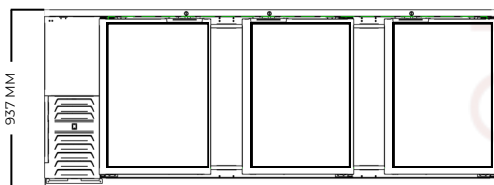
VISTA FRONTAL
