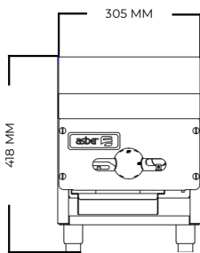
VISTA FRONTAL
