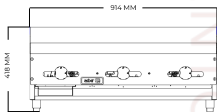
VISTA FRONTAL
