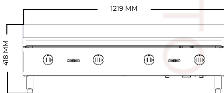
VISTA FRONTAL
