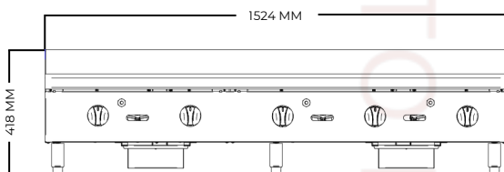
VISTA FRONTAL
