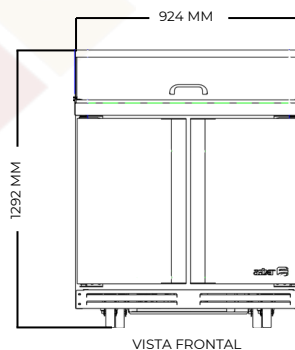
VISTA FRONTAL
