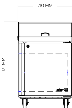
VISTA FRONTAL
