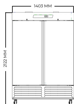
VISTA FRONTAL
